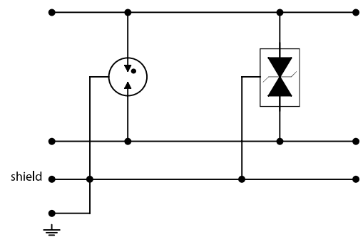
Basic circuit diagram
