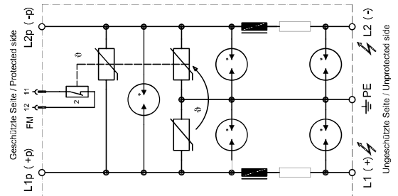
Basic circuit diagram
